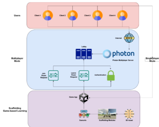
Fig. 2. Game-based learning architecture of scaffolding installation.
