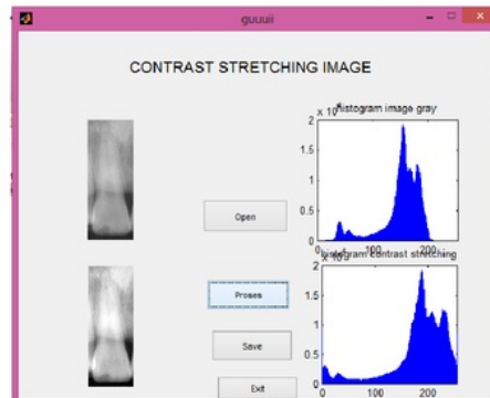
Gambar 7. Tampilan GUI proses contrast stretching
