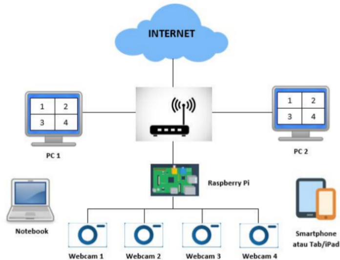
Fig. 1 Hardware Architecture
