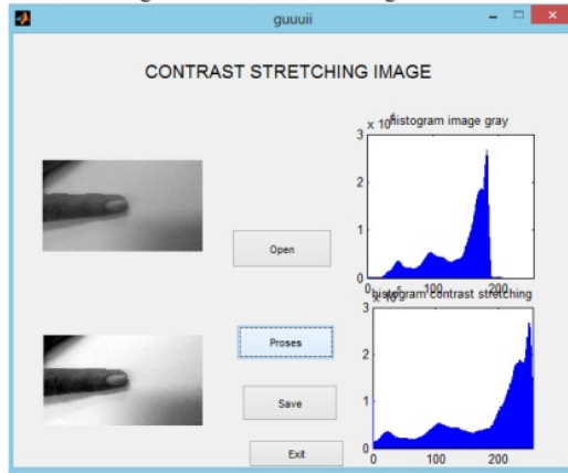
Figure 6. GUI of contrast stretching
