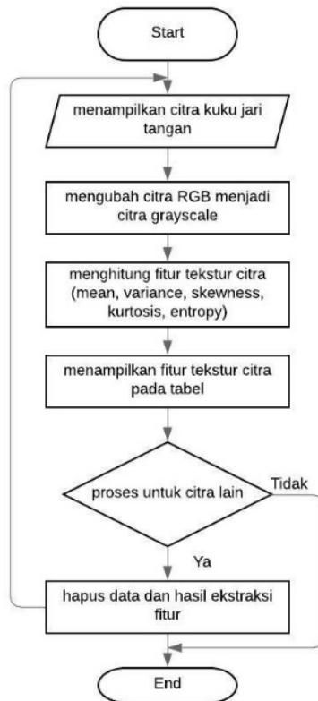
Gambar 6. Flowchart Program
