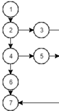
Figure 17. Flow graph of uric acid determination in application
