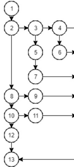
Figure 15. Flow graph of glucose determination in application
