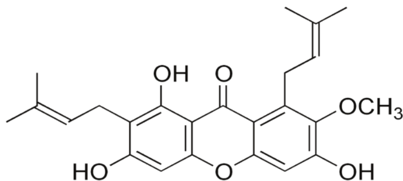
Fig. 1. Molecule structure of \alpha -mangosteen
