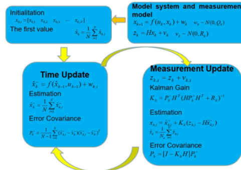
Figure 2. Square Root Ensemble Kalman Filter Algorithm [11].
