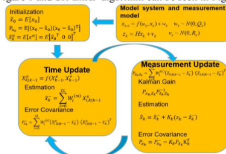
Figure 1. Unscented Kalman Filter Algorithm [4].
