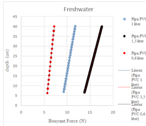
Figure 7. Graph of freshwater entering PVC pipe \geq \frac{3}{4} volume.
