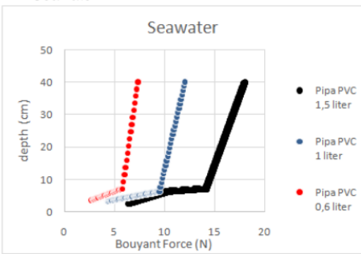
Figure 5. Graph of Seawater coming into PVC pipe
