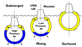
Figure 1. Flooding and Blowing of Ballast Systems
