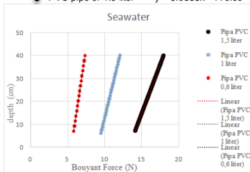
Figure 9. Graph of seawater entering PVC pipe \geq 3/4 volume
