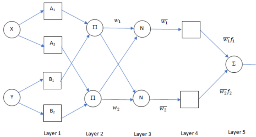
Figure 1. The diagram of ANFIS model
