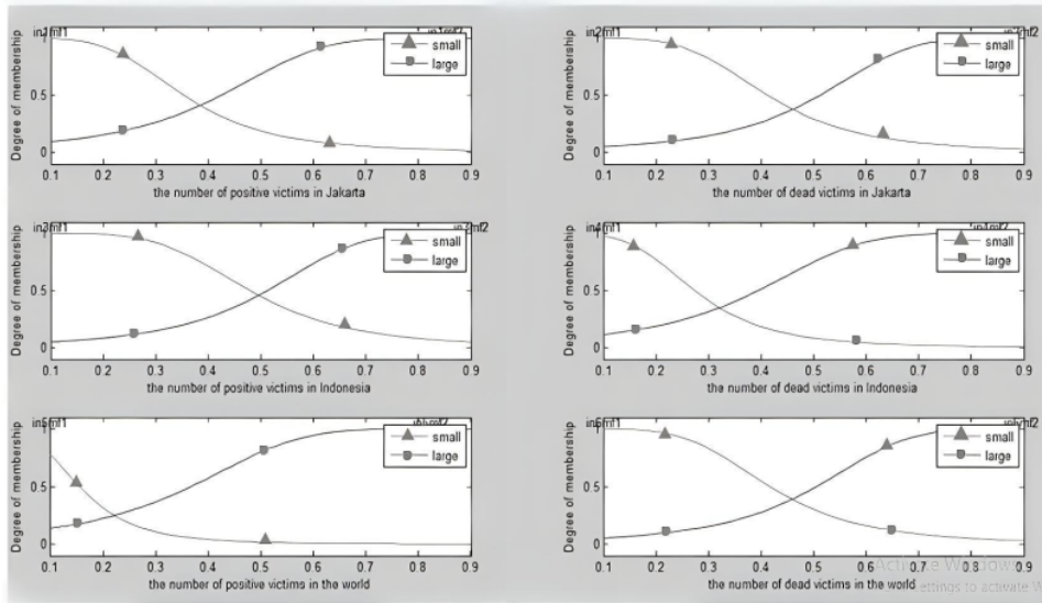
Figure 7. Optimal membership function of ANFIS
