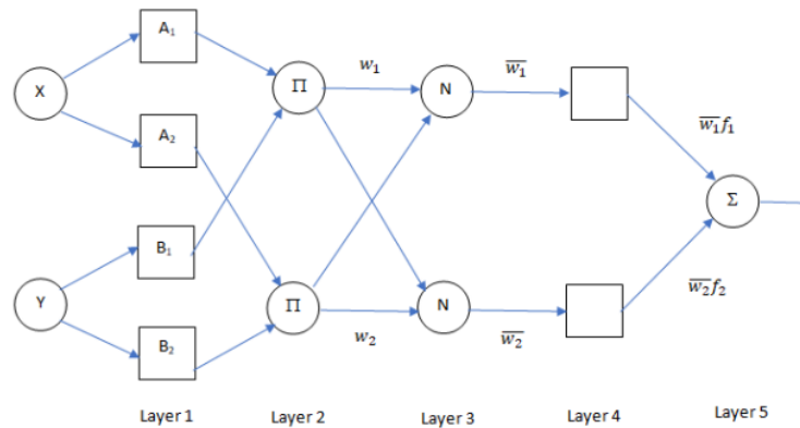
Figure 1. The diagram of ANFIS Model
