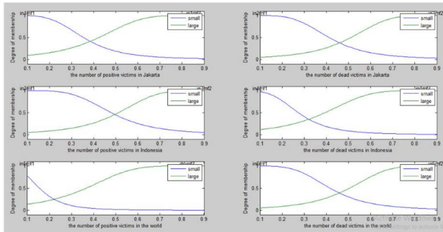
Figure 7. Optimal membership function of ANFIS
