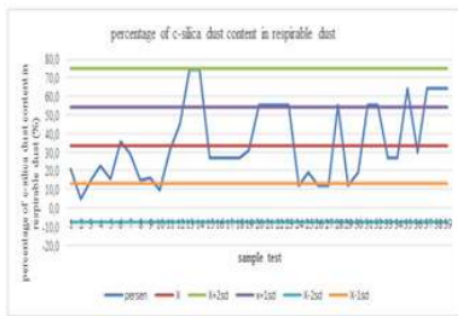
Figure 3. The Quality Control Chart Proportion of c-silica Dust Percentage in Respirable Dust.
