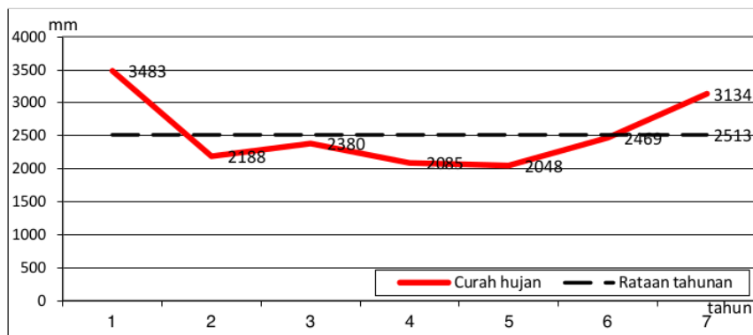
Fig. 1. Average annual rainfall for each period
