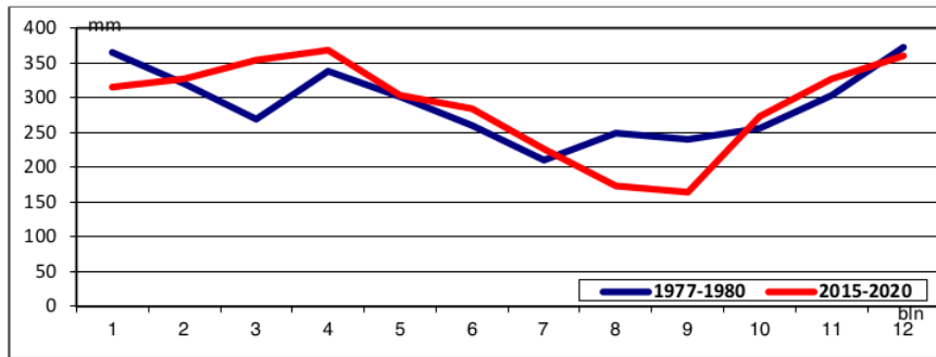
Fig. 2. Rainfall Pattern 1975-1980 and 2015-2019
