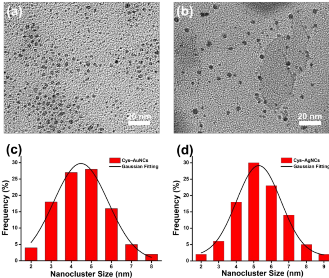
Figure 1. TEM images of the (a) Cys–AuNCs and (b) Cys–AgNCs. Histograms of the nanocluster size distributions and Gaussian fitting curves of the (c) Cys–AuNCs and (d) Cys–AgNCs.
