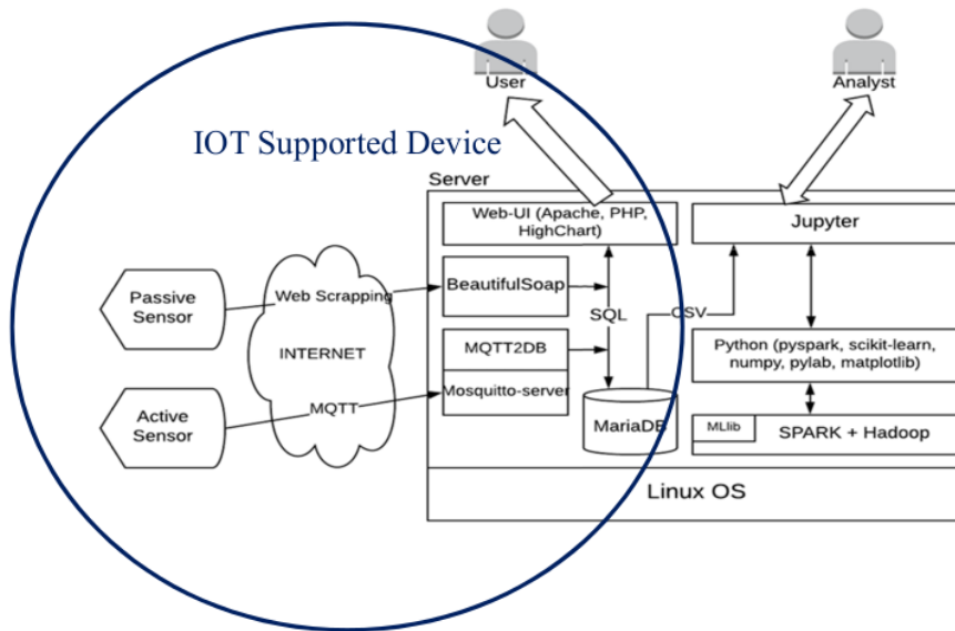
Fig. 1. System Design
