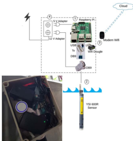
Fig. 4. Design Supported Sensor for IoT
