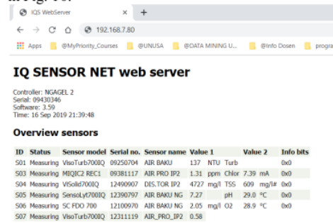
Fig. 10. Passive sensors web dashboard
