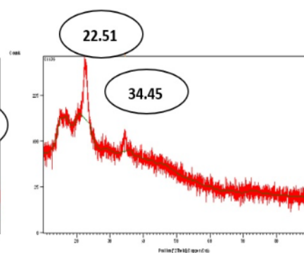
Figure 4. As-NP-BSA-CP XRD analysis
