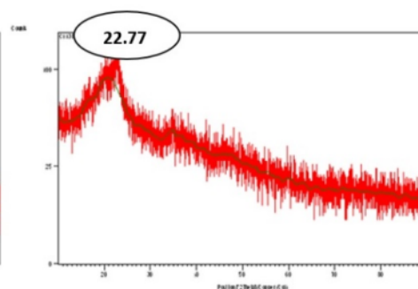
Figure 6. As-NP-BSA-Oh XRD analysis
