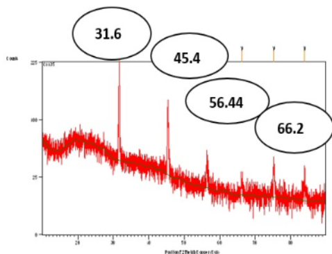
Figure 3. NP-BSA XRD analysis
