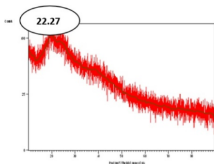
Figure 5. NP-BSA-Oh XRD analysis
